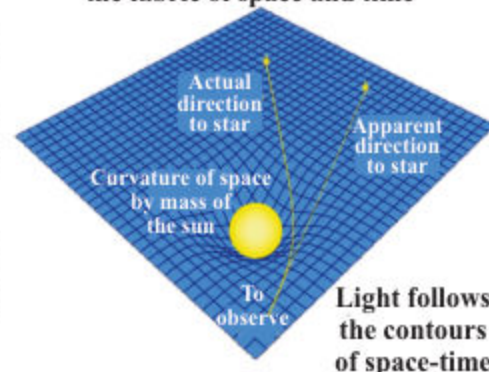
Figure 24. 16 Effects of Gravity
