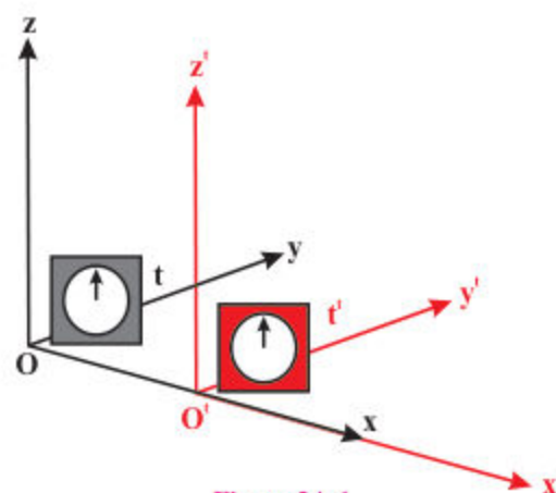
Figure 24.1 Cartesian Co-ordinate System
