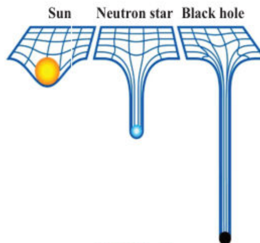
Figure 24. 14 Spacetime wrapping near heavy objects
