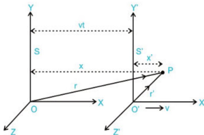
Figure 24.8 The Lorentz transformation
