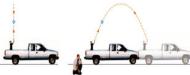
Figure 24.6: Principle of Relativity
