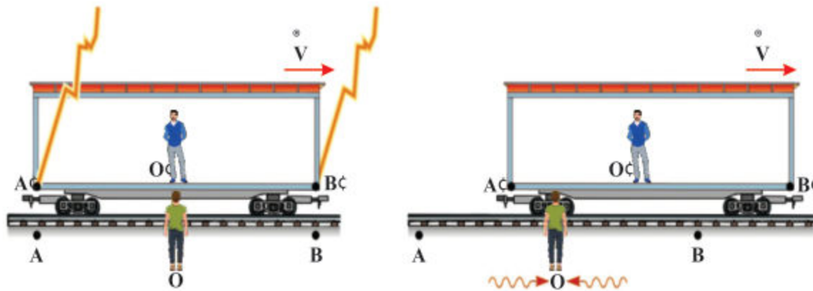
Figure 24. 9 Demonstration of Relativity of Simultaneity
