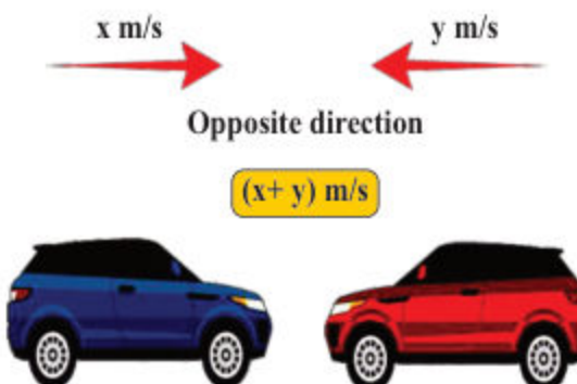
Figure 24.3 moving in different direction
