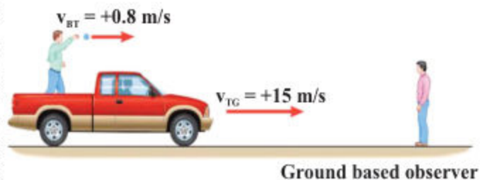
Figure 24.4: Moving and stationary frames of references
