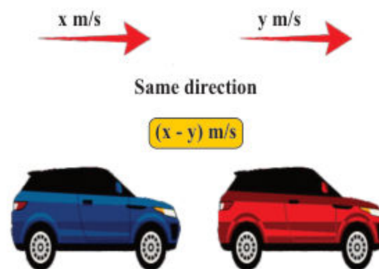
Figure 24.2 moving in same direction
